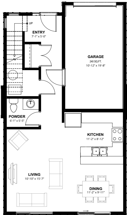
MAIN FLOOR 658 SQ.FT.
