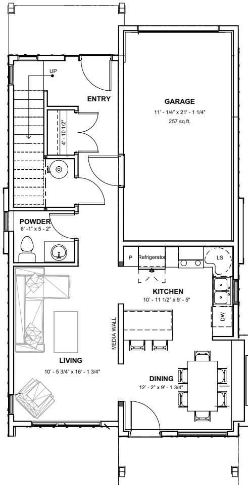
MAIN FLOOR 654 SQ.FT.
