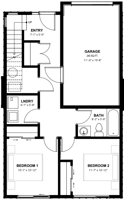
MAIN FLOOR 612 SQ.FT.
