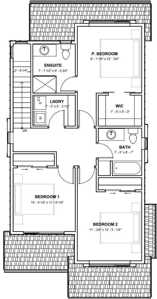
2ND FLOOR 855 SQ.FT.
