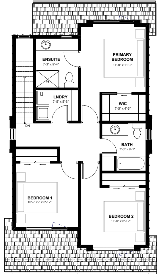
2ND FLOOR 819 SQ.FT.
